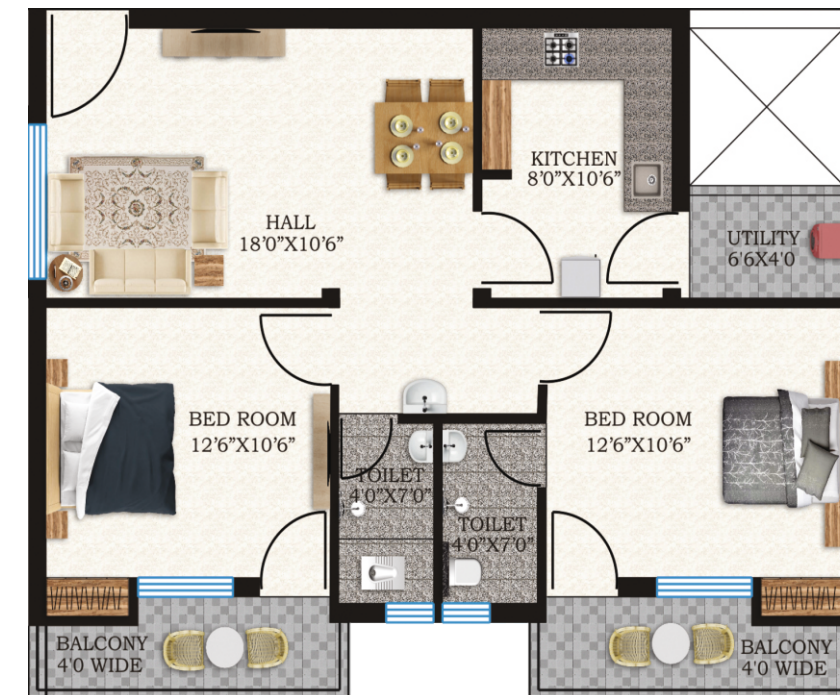
105-108 Typical Floor Plan
